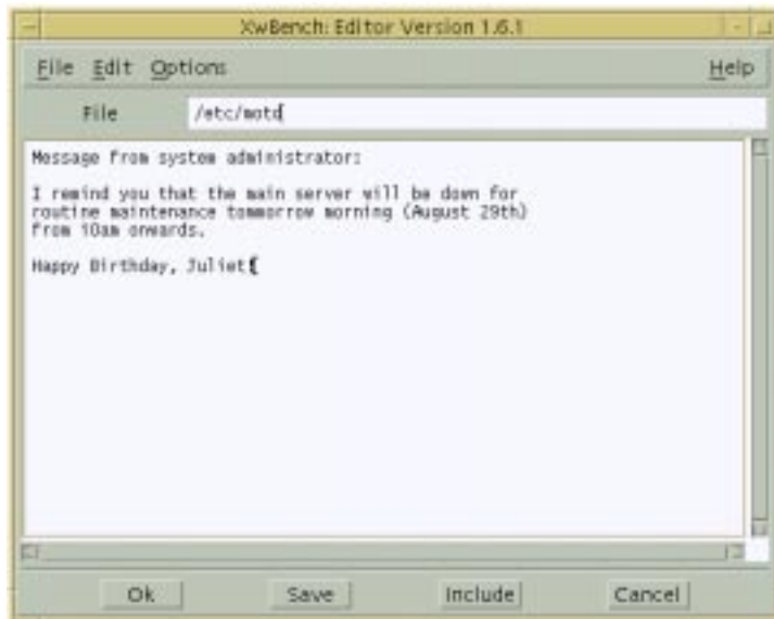
Figure 7-8 An editor dialog from a workbench application
