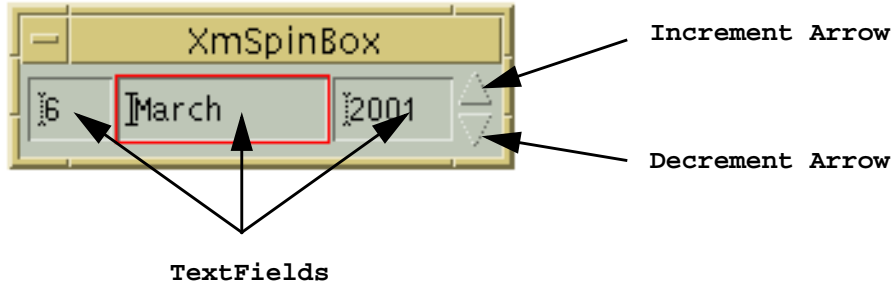
Figure 15-2 A SpinBox widget with three TextField children
