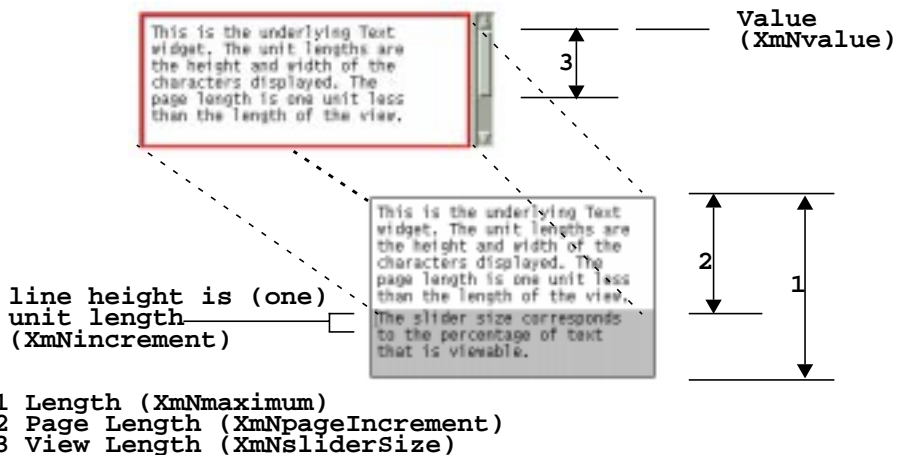
Figure 10-4 Conceptual relationship between ScrollBar and the object that it scrolls
