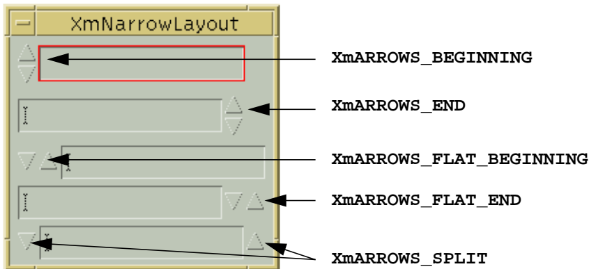
Figure 15-5 The various settings of the XmNarrowLayout resource
