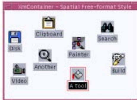
Figure 9-4 A Container in Spatial layout using coordinate placement
