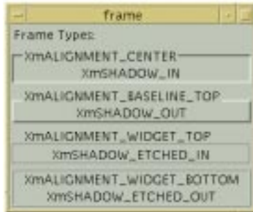
Figure 8-19 Output of the frame program
