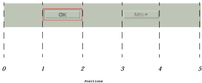
Figure 7-6 The XmNfractionBase resource divides the form into equal units
