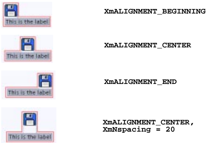
Figure 9-6 The effect of IconGadget alignment and spacing resources
